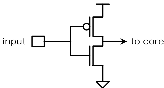
Figure 4.4 – Single-ended Receiver
