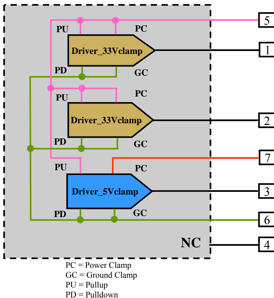
Figure 5.22 – Component Diagram Showing Buffer and Supply Buses
