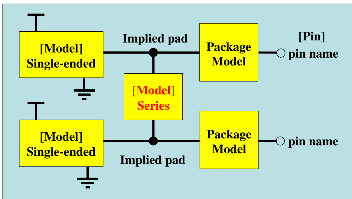
Figure 5.23 – Connection of Single-ended and Series [Model]s
