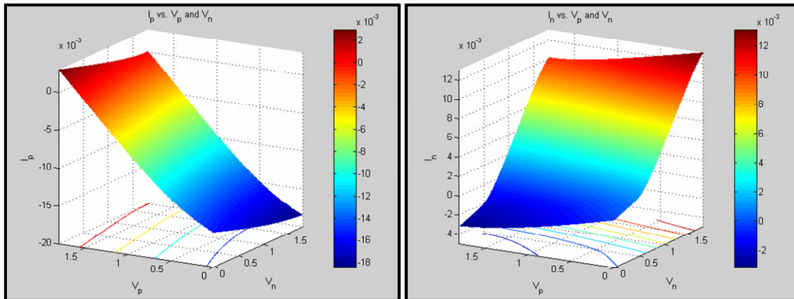
Figure 4.14 – Surface Plots of Raw Data from I-V Sweep of Differential Buffer
