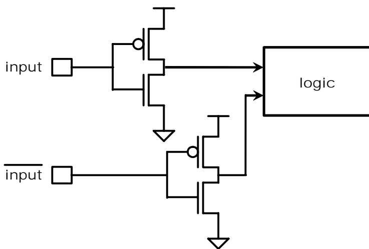
Figure 4.7 – Pseudo-differential Receiver
