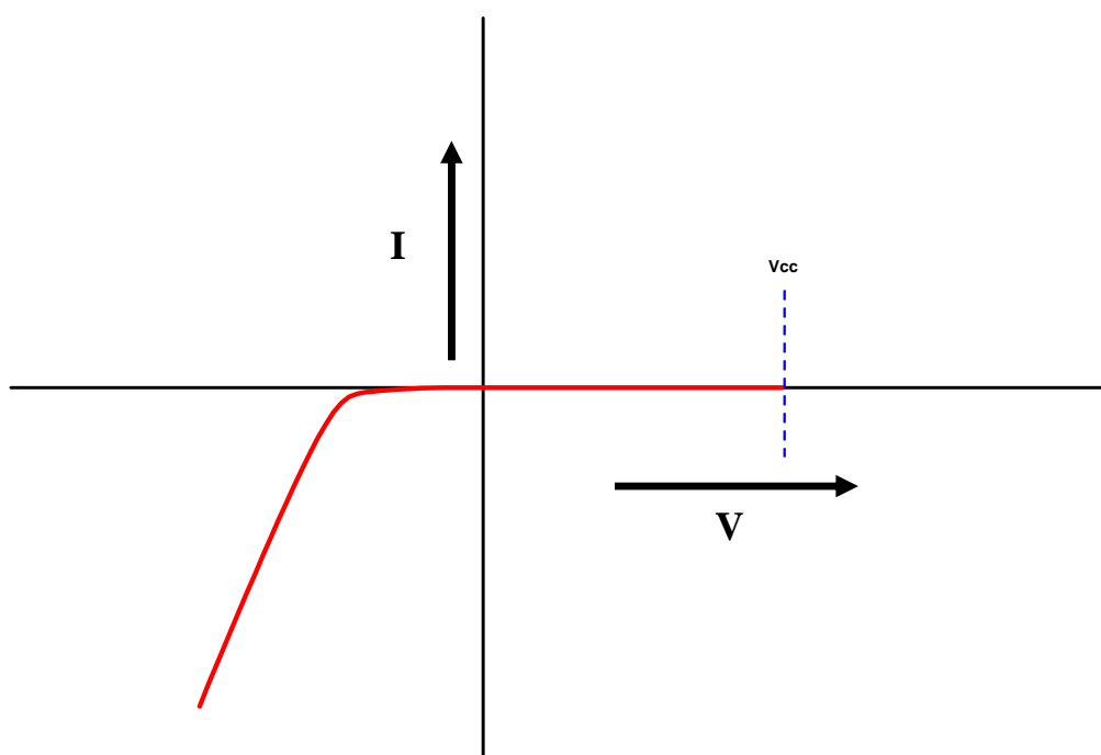
Figure 5.4 – Graph of [GND Clamp] I-V Table Data
