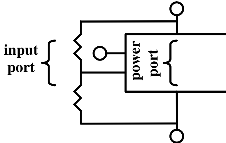
Figure 3.5 – Input Port with Locally Generated Reference
