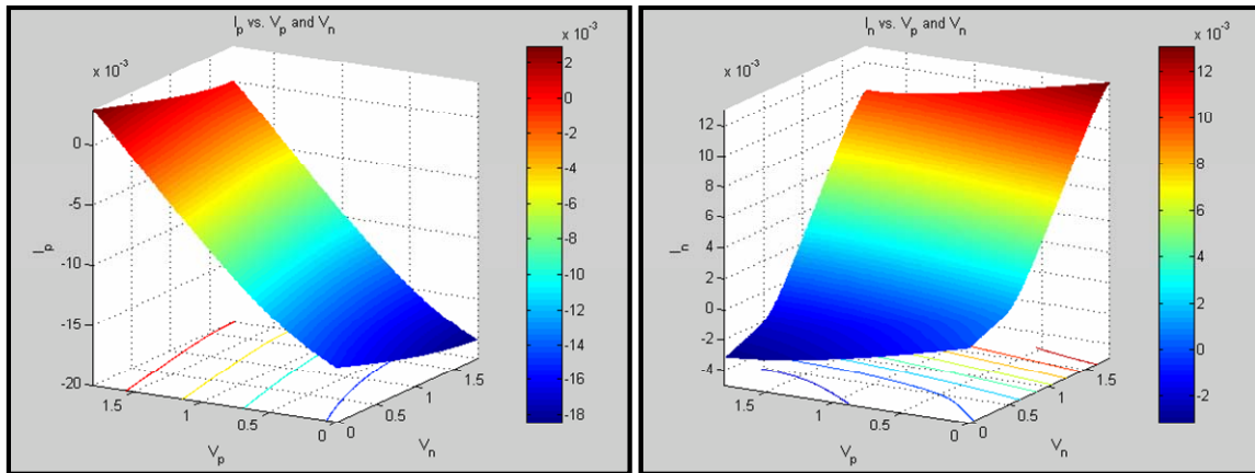
Figure 3.16 - Surface Plots of Raw Data from I-V Sweep of Differential Buffer
