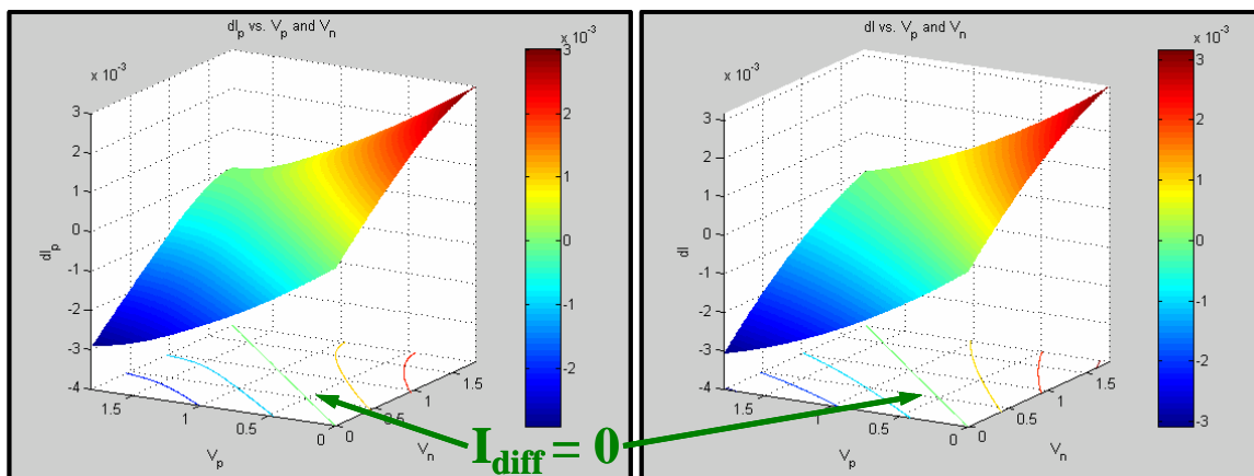
Figure 3.18 – Differential Current Plot of Output Current versus P and N Voltage
