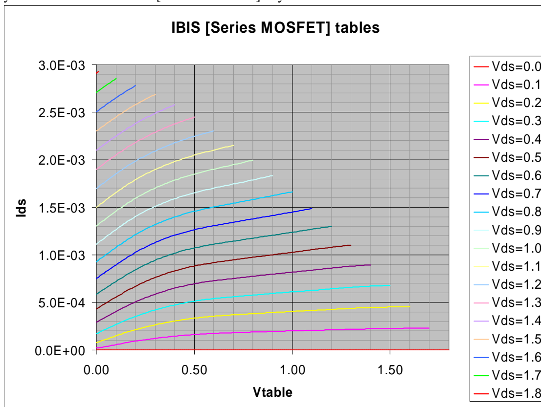
Figure 3.19 - Plots of Various V_{ds} Values for a [Series MOSFET] Buffer
