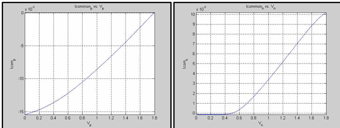
Figure 3.17 - I-V Curves of Common Mode Characteristics of Differential Buffer
