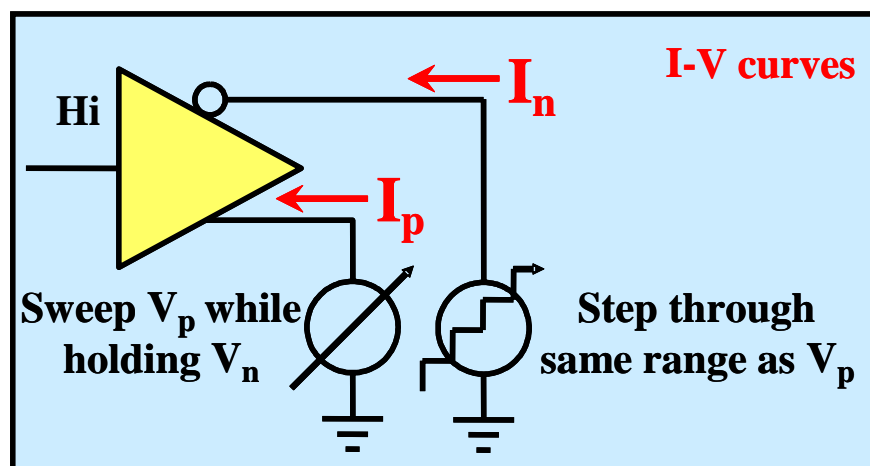
Figure 3.15 - I-V Table Extraction Fixture for a Differential Buffer
