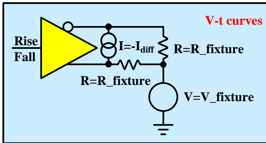
Figure 3.20 – V-T Table Extraction Fixture for a Differential Buffer
