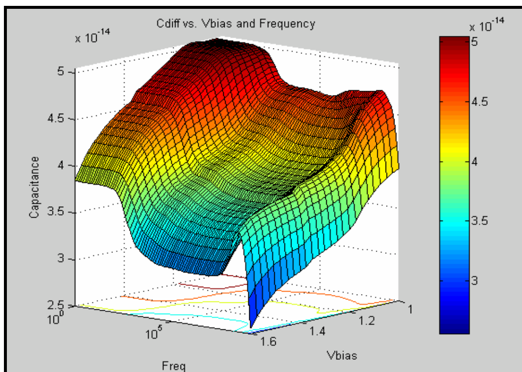
Figure 3.26 - Surface Plot of Differential Capacitance versus Frequency and DC Bias Voltage
