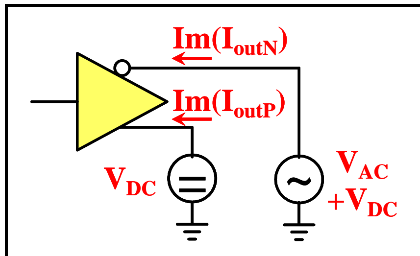
Figure 3.25 - Fixture for Extraction of Differential Buffer C_{comp}
