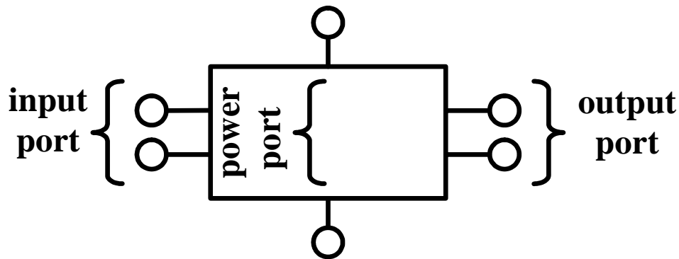
Figure 3.3 – Device with Independent Input, Output and Power Supply Ports
