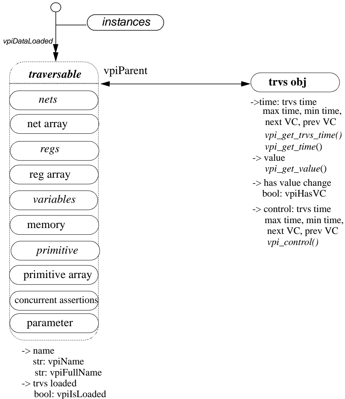
Figure 29-2 — Model diagram of traverse object
