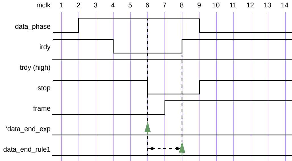
Figure 17-14 — Conditional sequences
