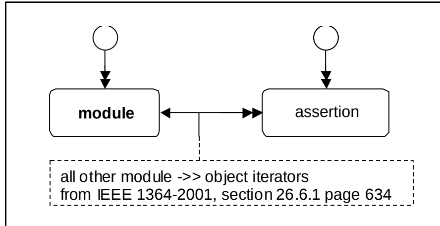
Figure 27-1 — Encompassing assertions
