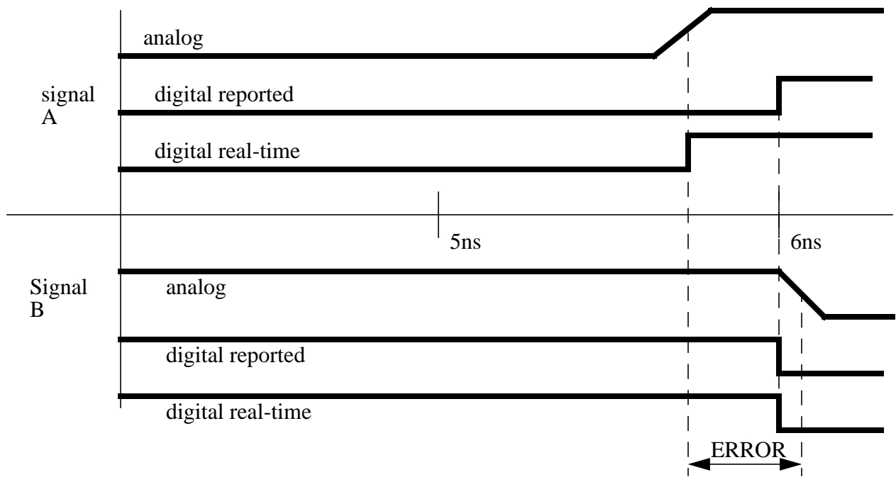
Figure 8-1: Rounding of A2D events
