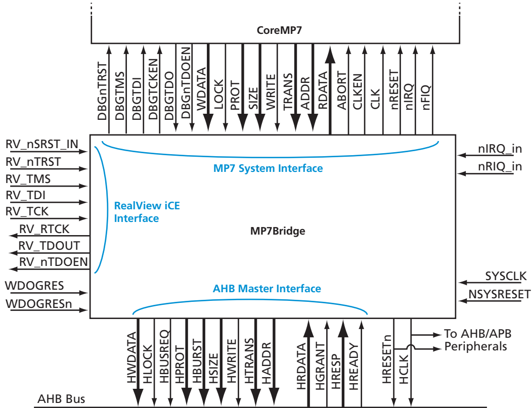
Figure 2 • CoreMP7Bridge Connection
