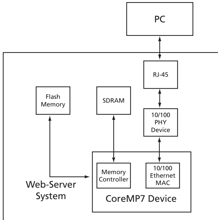
Figure 1 • Web Server Block Diagram
