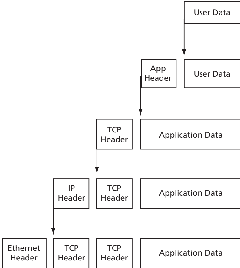
Figure 2 • TCP/IP Packet Encapsulation
