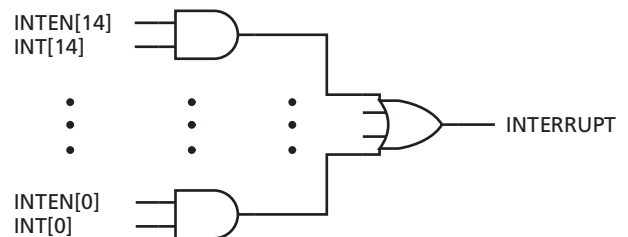
Figure 4 • CoreAI Interrupt Logic
