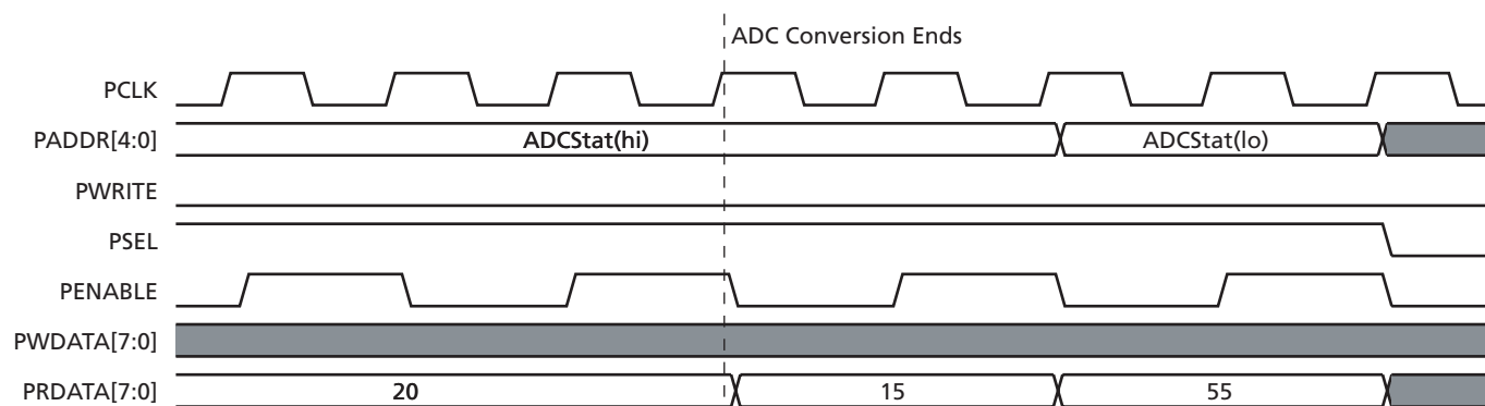
Figure 8 • ADC End of Conversion
