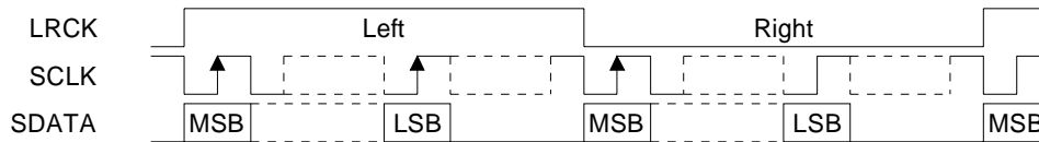
Figure 36. Left Justified Format
