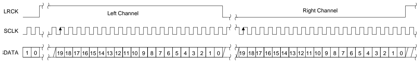
Figure 13. Format 4, Right Justified 20-Bit Data. (Available in Control Port Mode only)
