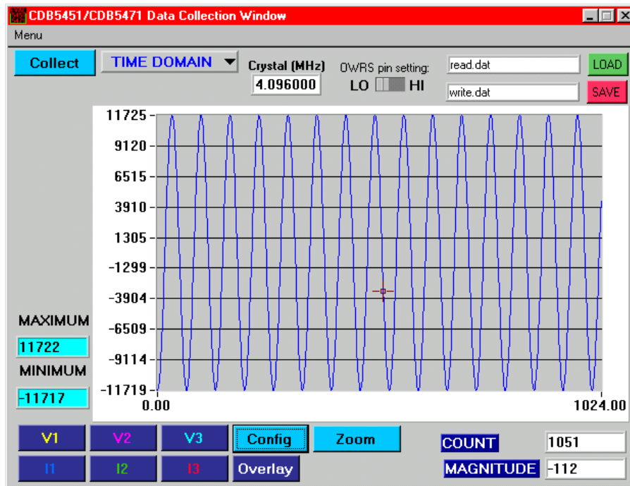
Figure 6. Data Collection Window (Time Domain)
