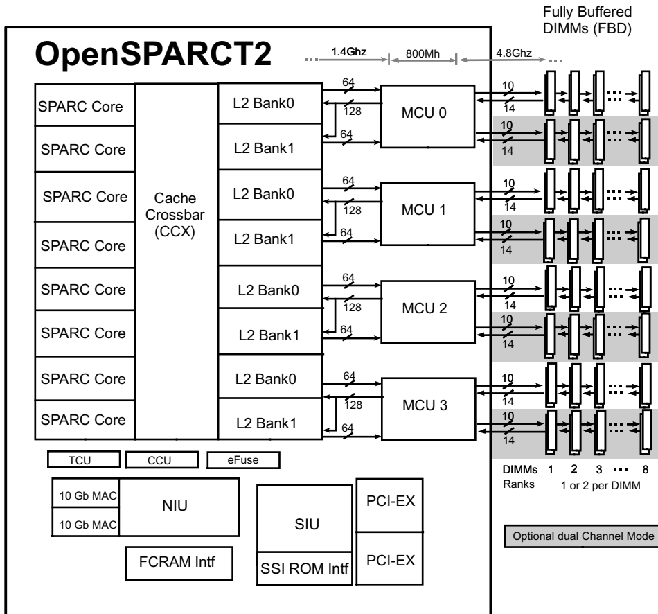
FIGURE 2-1 OpenSPARC T2 Chip Block Diagram
