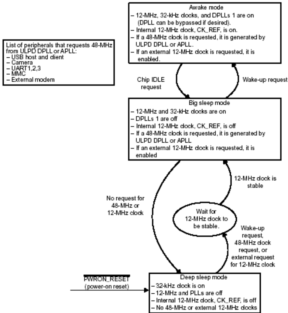
Figure 4. Power Management Mode Transitions
