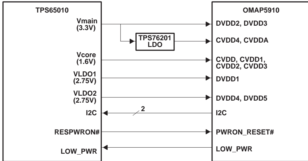
Figure 3. OMAP Low-Power System Architecture
