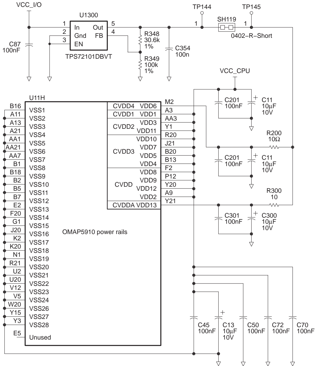
Figure 5. OMAP5910 Core/PLL Voltages
