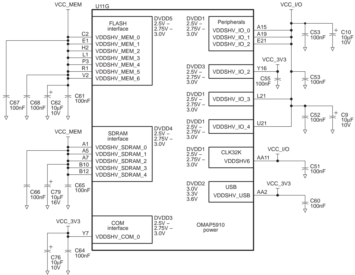
Figure 6. OMAP5910 I/O, Memory and USB Voltages
