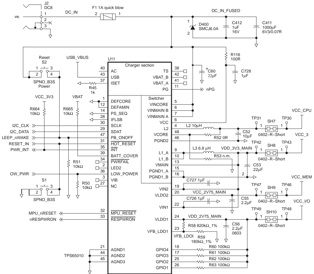
Figure 7. TPS65010 Power Management Circuit
