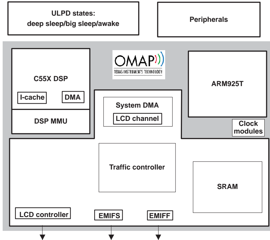
Figure 1. OMAP5910 Device Architecture
