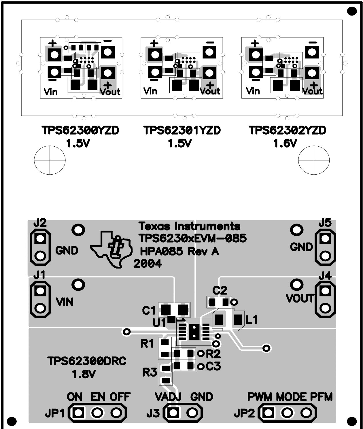
Figure 3. Assembly Layer
