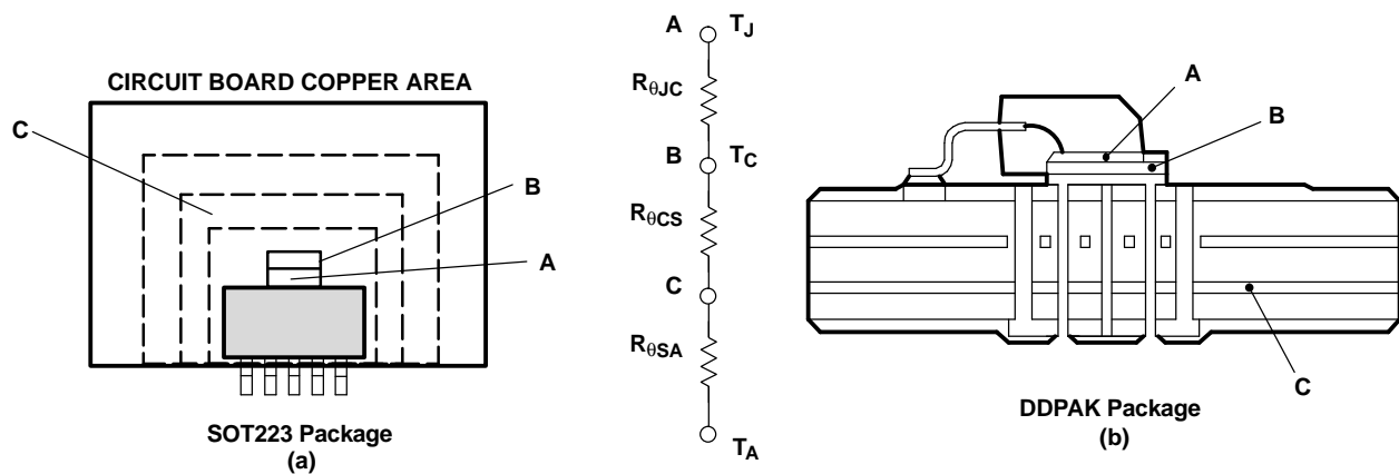
Figure 24. Thermal Resistances
