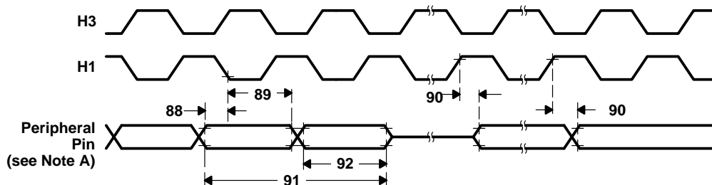
Figure 31. Timing for Timer Pin
