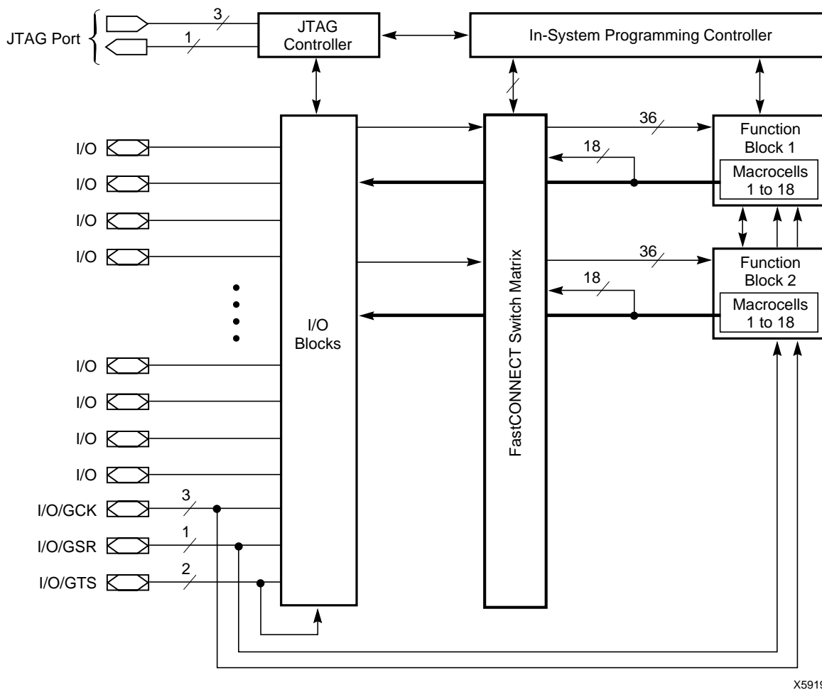
Figure 2: XC9536 Architecture
