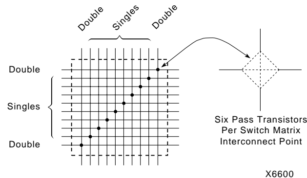
Figure 27: Programmable Switch Matrix (PSM)
