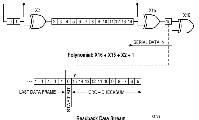
Figure 46: Circuit for Generating CRC-16
