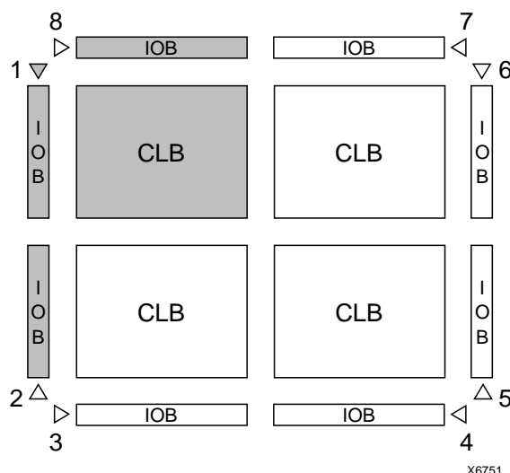
Figure 38: Left and Right BUFGEs Can Drive Any or All Clock Inputs in Same Quadrant or Edge (GCK1 is shown. GCK2, GCK5 and GCK6 are similar.)
