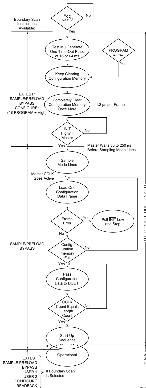
Figure 47: Power-up Configuration Sequence
