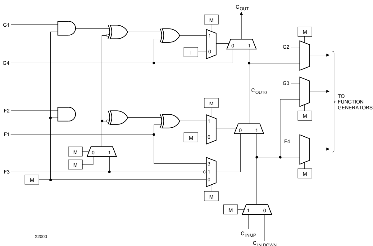
Figure 15: Detail of XC4000E Dedicated Carry Logic
