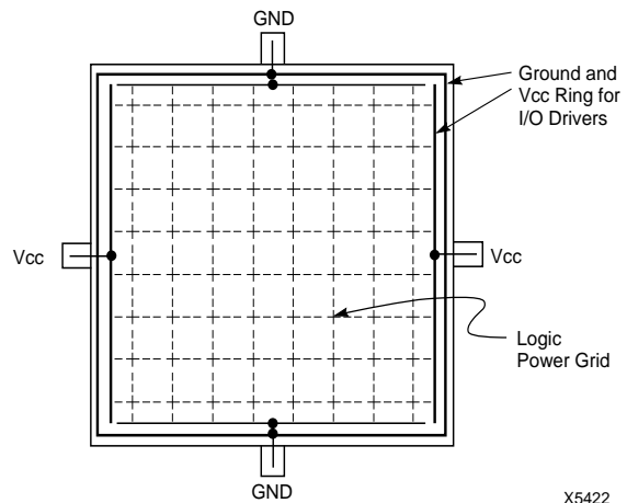
Figure 40: XC4000 Series Power Distribution
