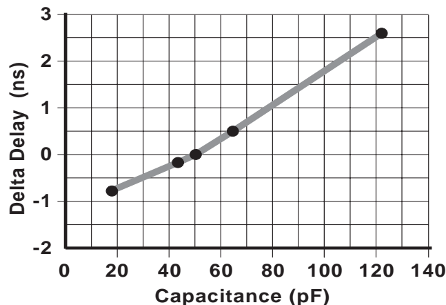
Figure 61: Additional Delay VS Capacitive Loads
