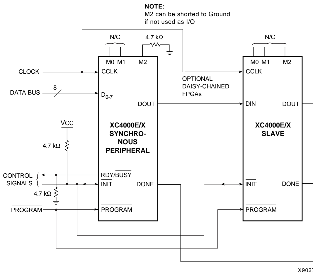
Figure 57: Synchronous Peripheral Mode Circuit Diagram
