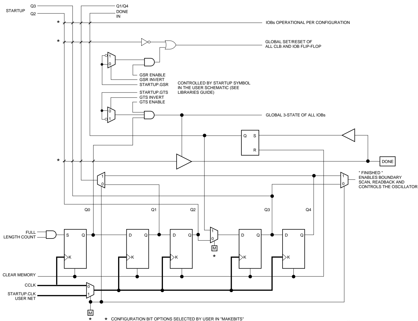
Figure 49: Start-up Logic
