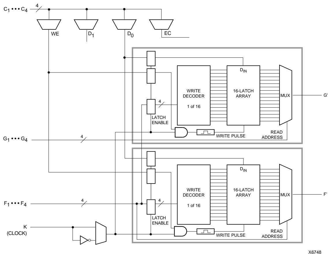
Figure 8: 16x1 Edge-Triggered Dual-Port RAM
