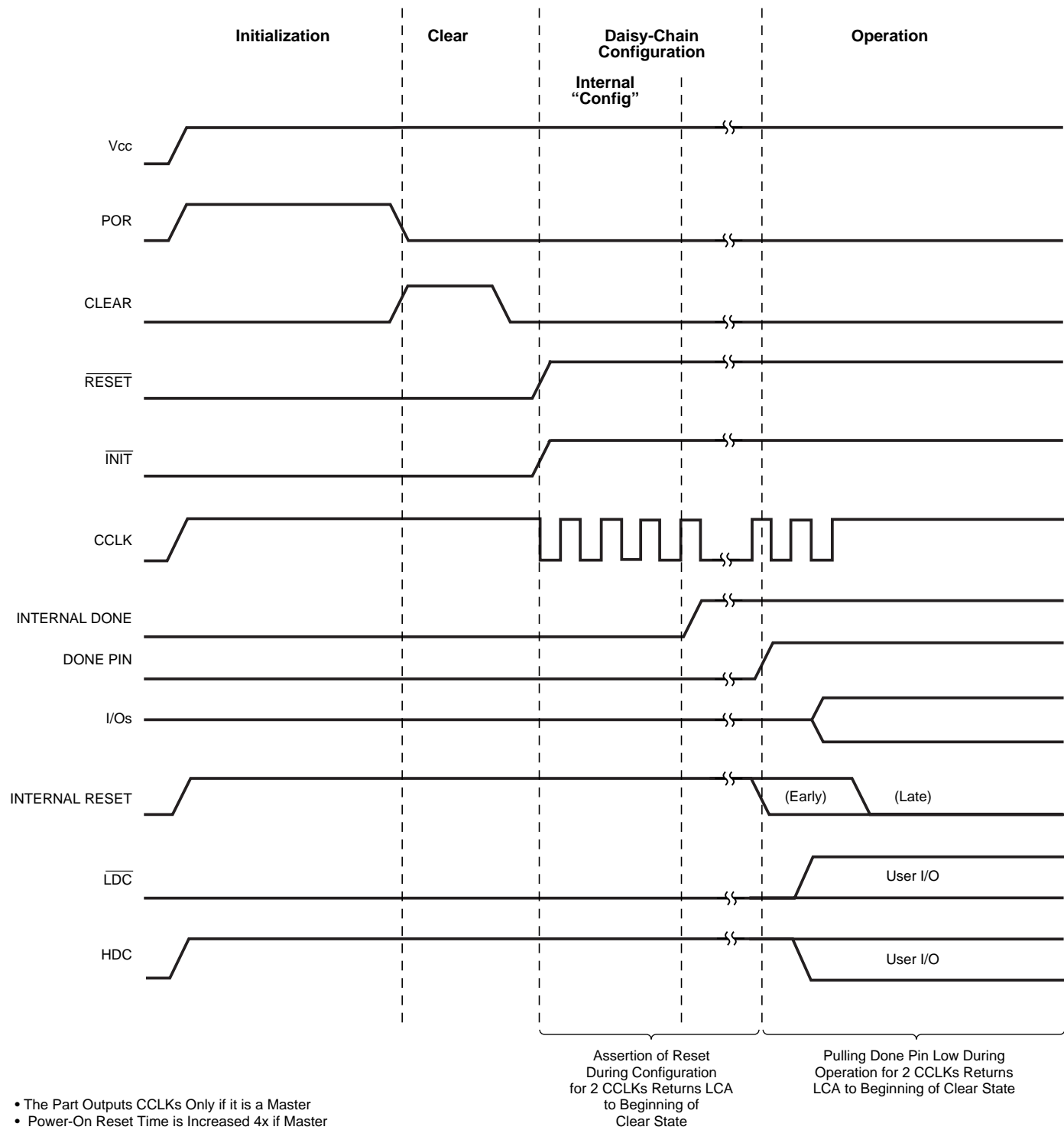
Figure 4. Psuedo-Configuration Waveform (Configuration Delay by Reset )
