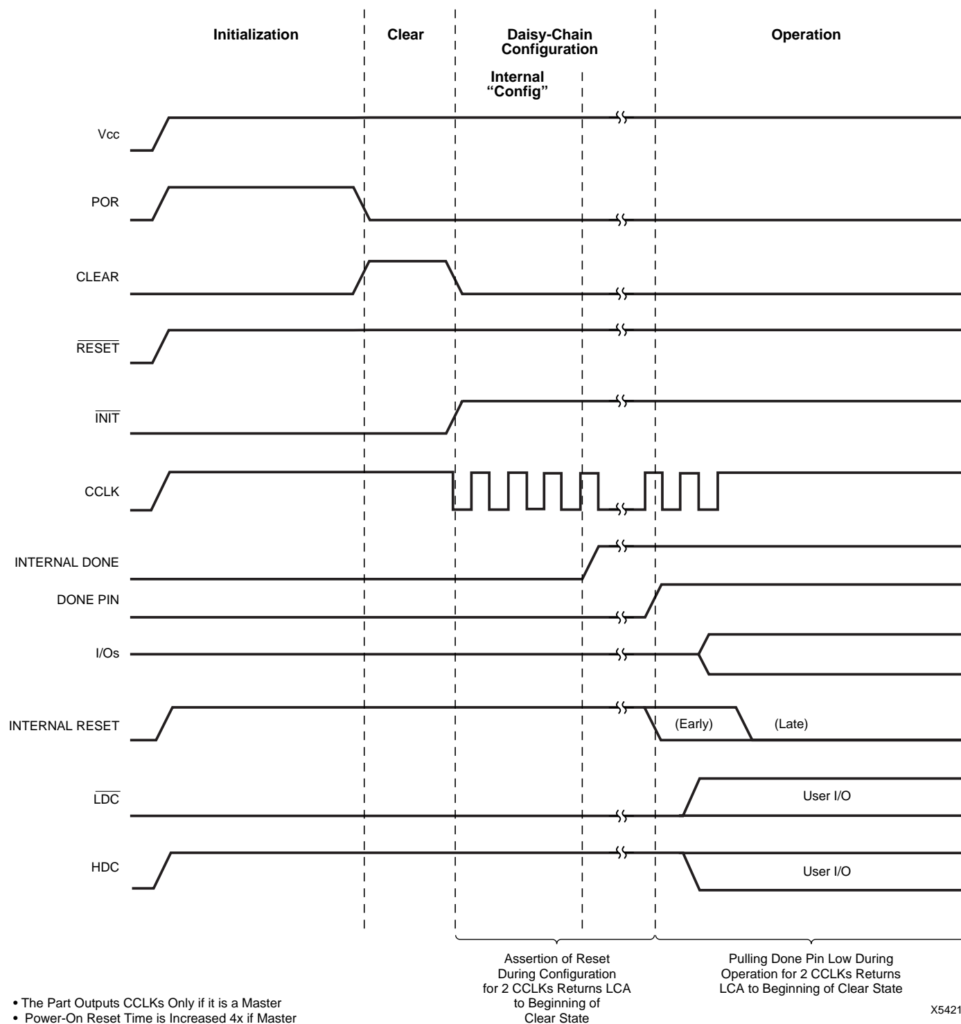
Figure 3. Psuedo-Configuration Waveform (Normal Power-Up)
