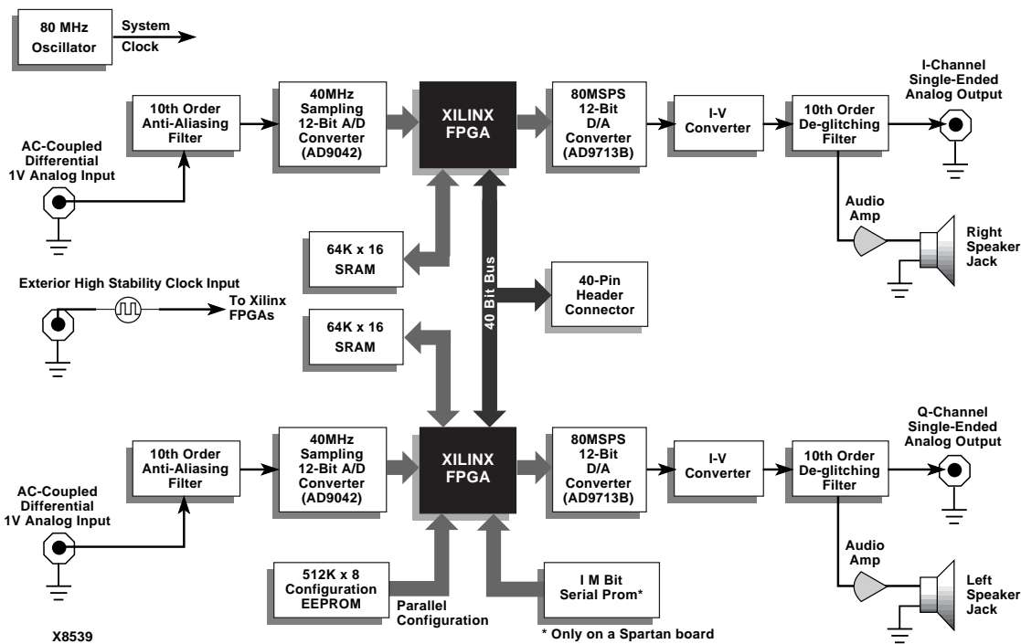
Figure 1: GVA-200 Block Diagram
