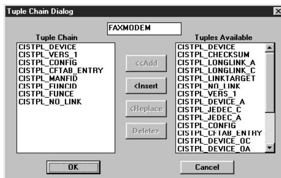
Figure 1: Tuple Chain Dialog Box
