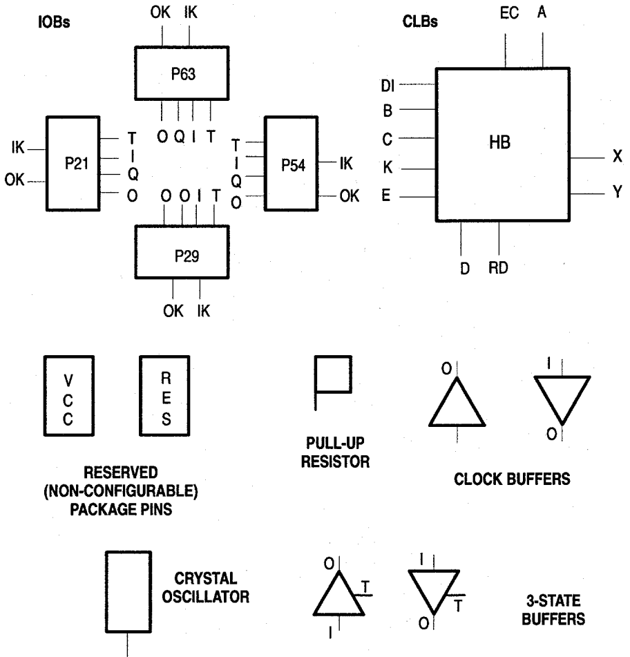
Figure 4-3 Block Inputs and Outputs (XC3000)
