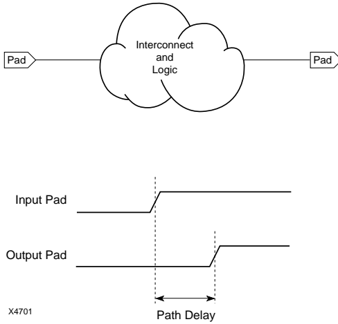
Figure 1-1 Pad To Pad Path
