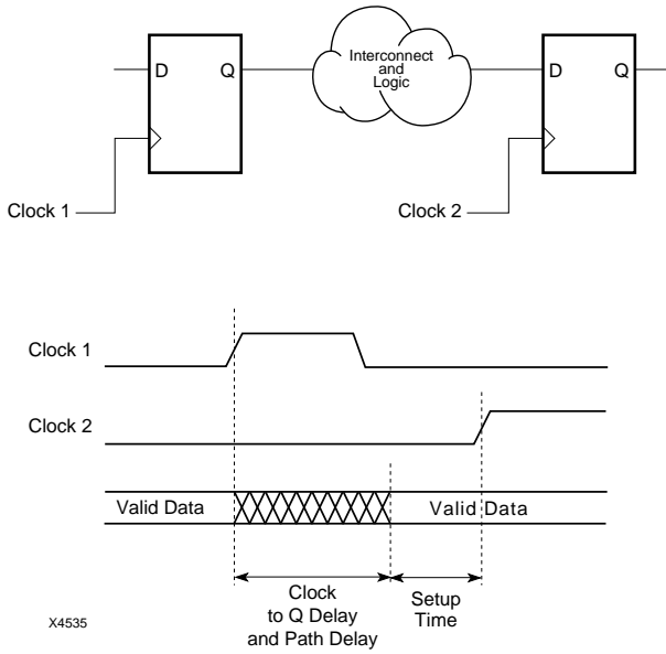
Figure 1-5 Clock To Setup Path, Different Clock Net
