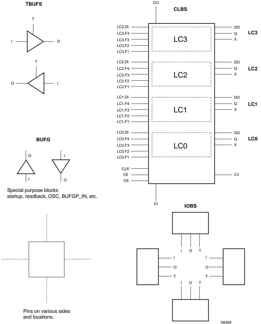
Figure 4-5 Block Inputs and Outputs (XC5200)
