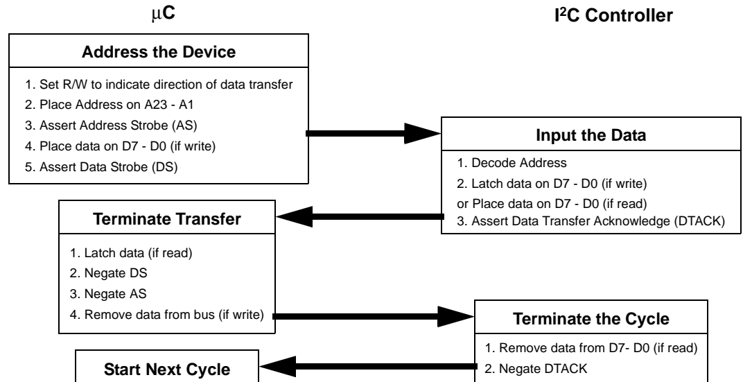
Figure 4: \mu\text{C} Read/Write Protocol
