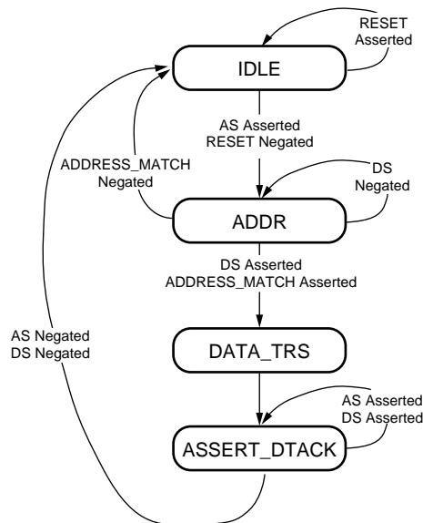
Figure 5: \mu\text{C} Bus Interface State Machine
