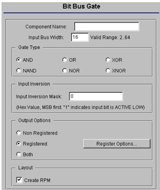
Figure 1: Main Bus Gate Parameterization Screen
