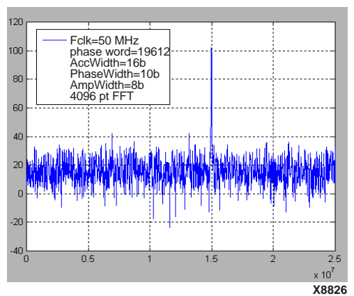
Figure 8: Power Spectral Density, 15 MHz Tone
