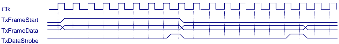
Figure 4: System Interface Transmit Timing 1
