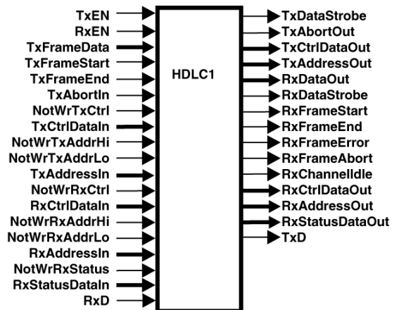
Figure 1: Core Schematic Symbol
