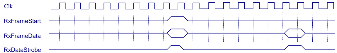
Figure 6: System Interface Receive 1
