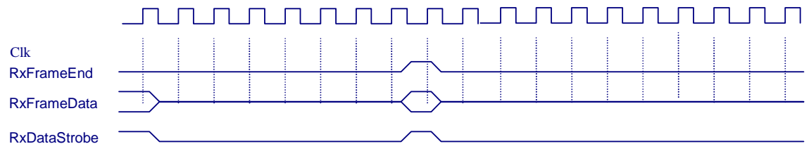
Figure 7: System Interface Receive 2
