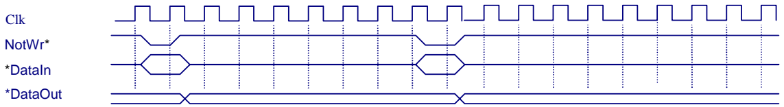
Figure 8: Register Interface Timing
