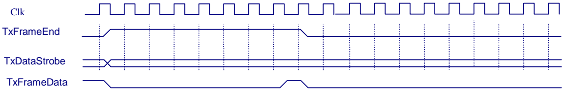
Figure 5: System Interface Transmit Timing 2
