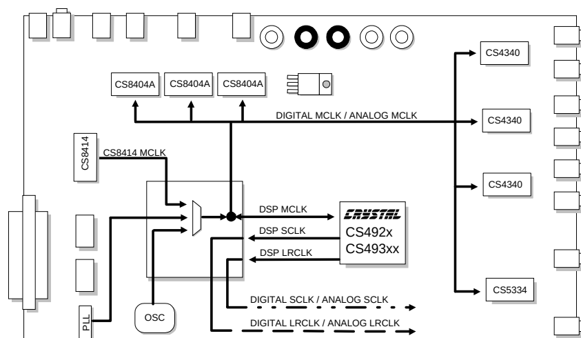
Figure 3. Audio Clocking
