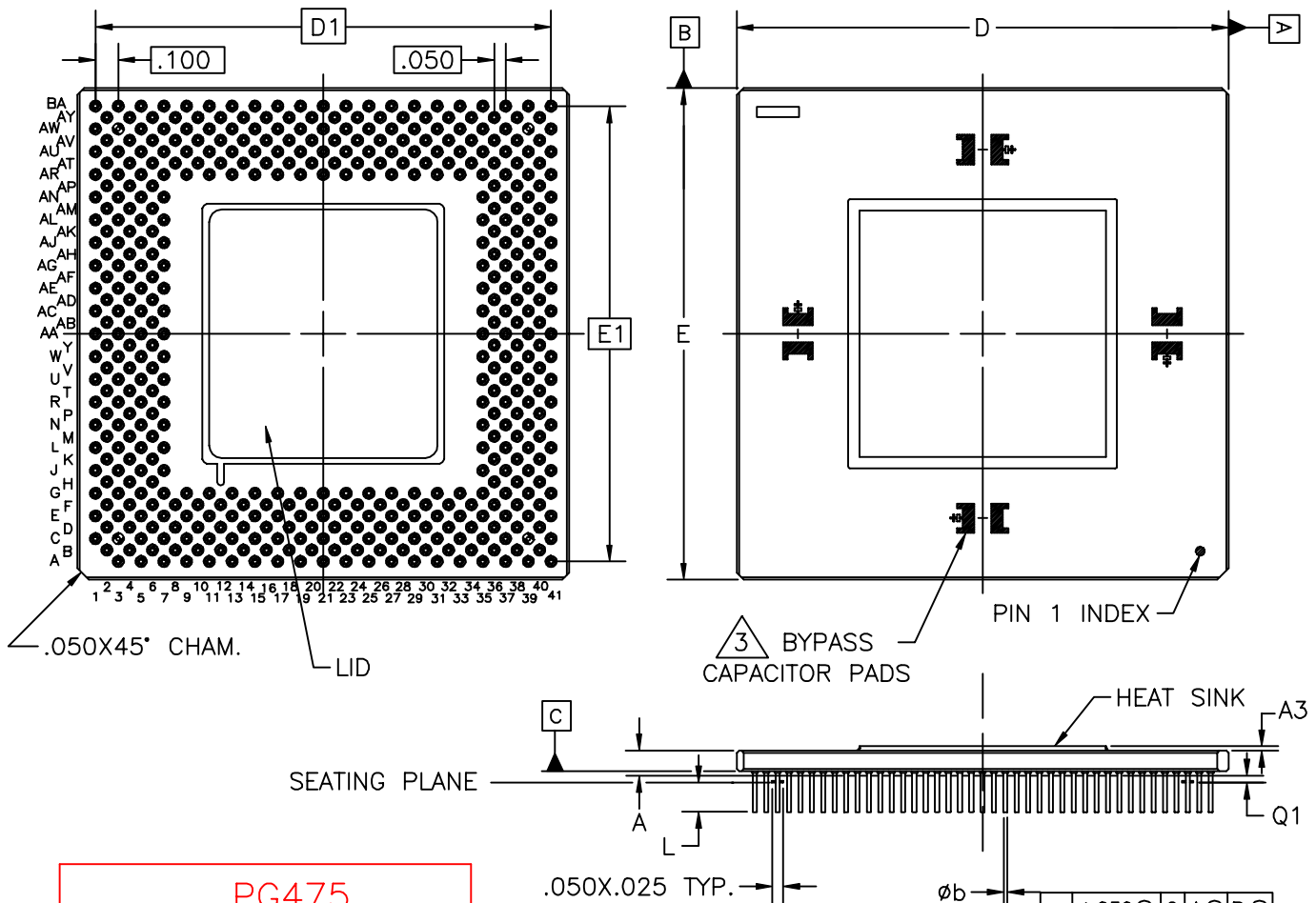
BOTTOM VIEW
