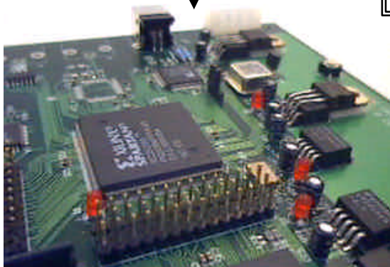
Mentor Graphics USB 2.0 Transfer System Board
