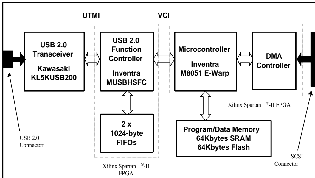
USB 2.0 Transfer System Block Diagram
