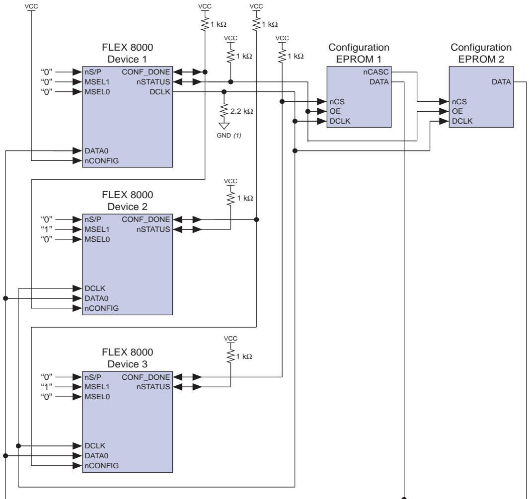
Figure 1. Multi-Device Sequential Active Serial (MD-SAS) Configuration Circuit
