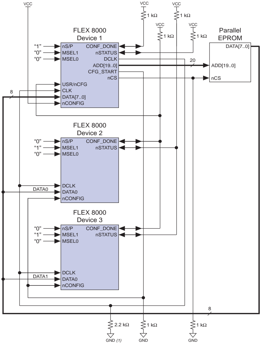
Figure 10. Multi-Device Active Parallel Hybrid (MD-APH) Configuration Circuit
