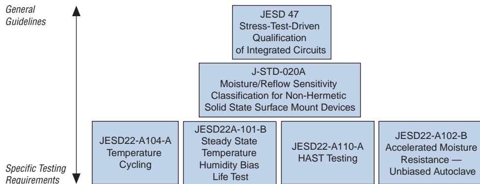
Figure 1. EIA/JEDEC Testing Hierarchy
