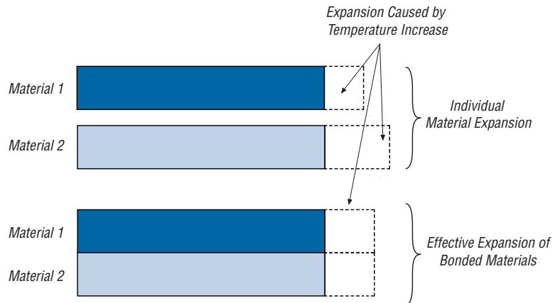
Figure 2. The Effects of Thermal Coefficient of Expansion on Two Materials
