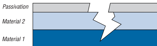
Figure 3. Passivation Cracking & Layer Displacement
