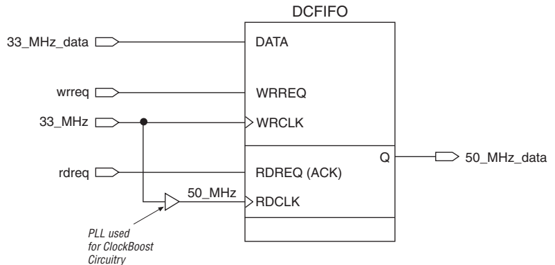
Figure 24. Using DCFIFO to Interface between Clock Domains
