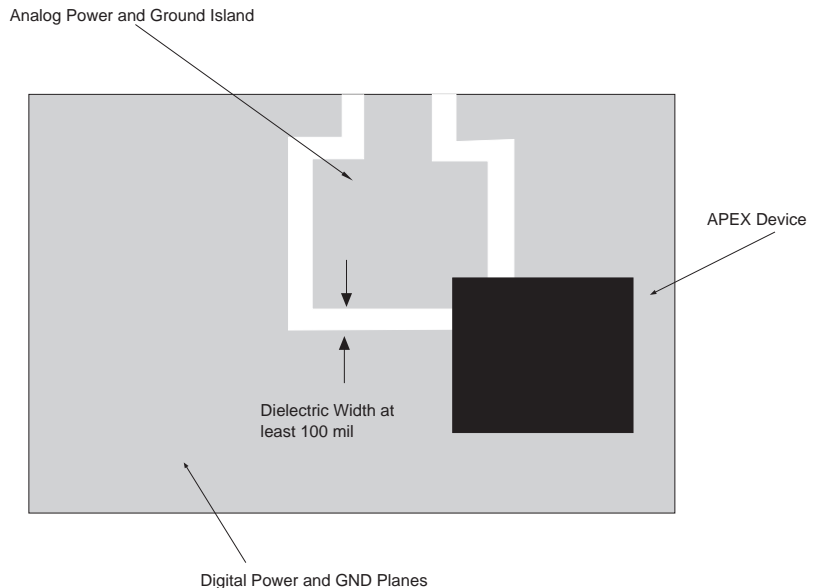
Figure 9. Board Layout for PLL VCC and GND Islands
