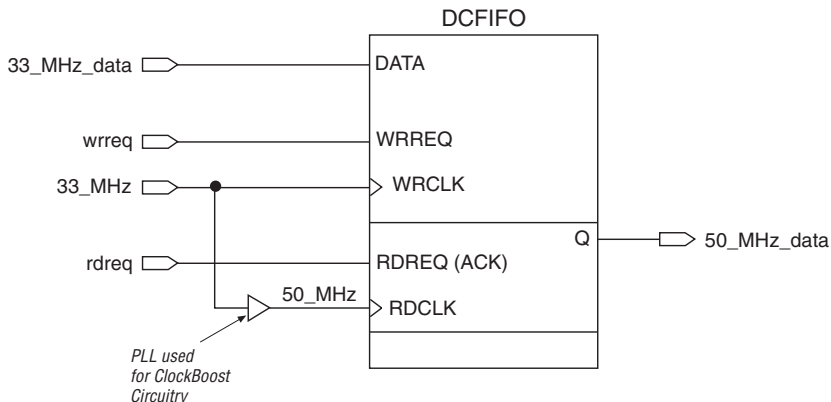
Figure 17. Using DCFIFO to Interface between Asynchronous Clock Domains
