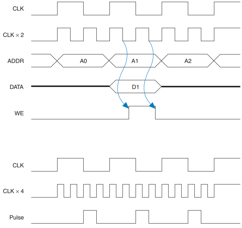
Figure 20. Using Multiplication to Generate Pulses
