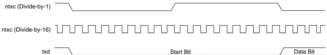
Figure 6. Transmitter Data & Clock Signals
