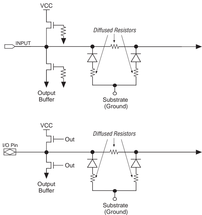
Figure 2. Altera Device Input Protection Structures
