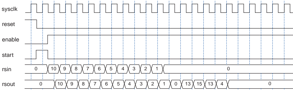
Figure 2. Continuous Encoding
