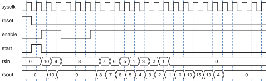
Figure 1. Discrete Encoding
