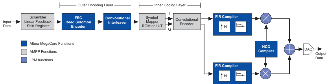
Figure 2. Typical Modulator
