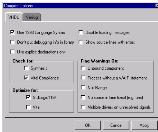
Figure 7. Compiler Options
