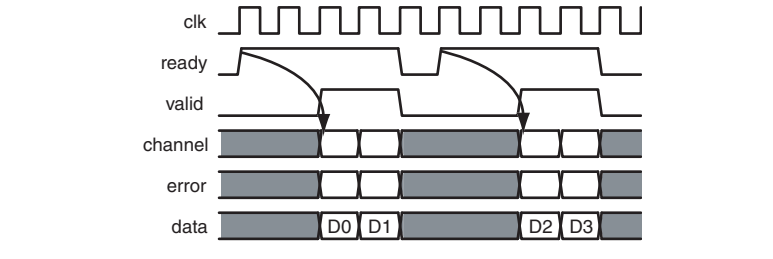
Figure 6.8. Transfer with Backpressure, readyLatency=2
