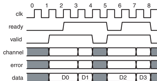
Figure 6.6. Transfer with Backpressure, readyLatency=0
