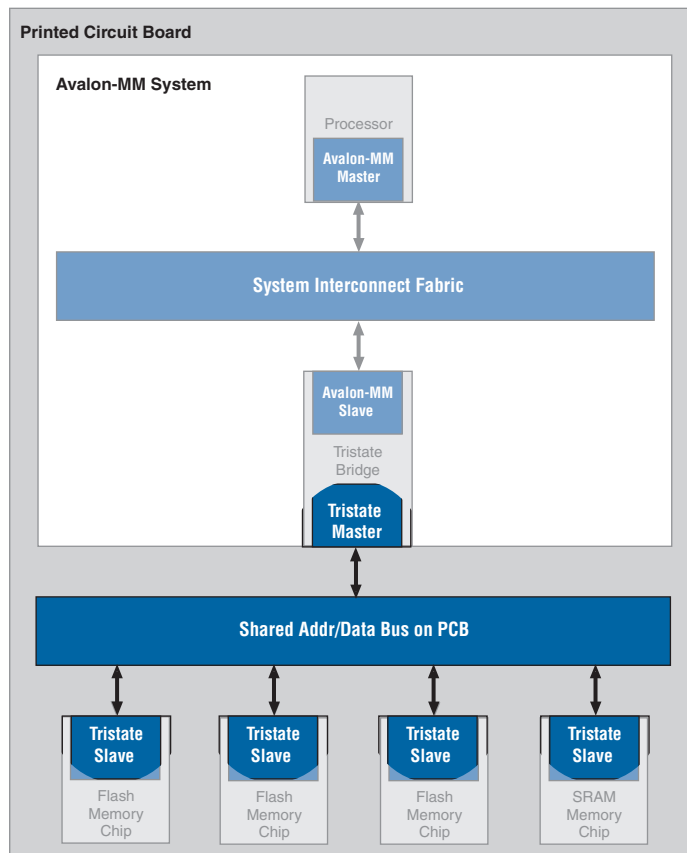
Figure 5.1. Typical Use of Avalon-MM Tristate Interface
