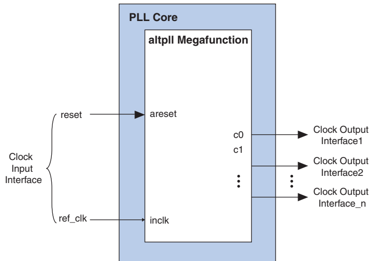
Figure 2.1. PLL Core Clock Outputs and Inputs
