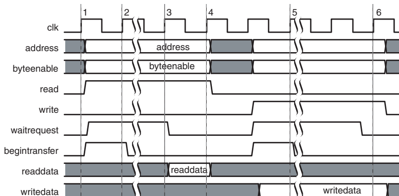
Figure 3.3. Slave Read and Write Transfers with Peripheral-Controlled Waitrequest
