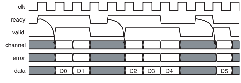
Figure 6.7. Transfer with Backpressure, readyLatency=1
