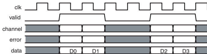
Figure 6.5. Data Transfer without Backpressure
