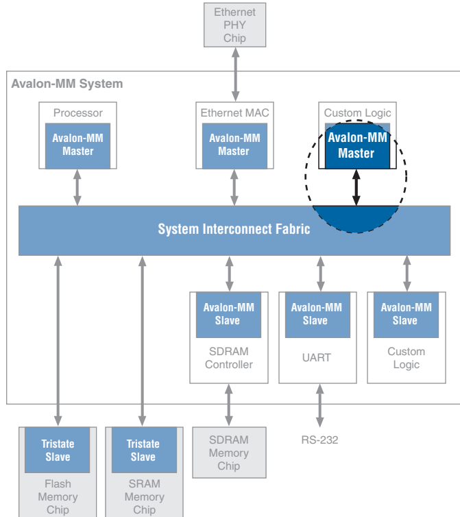
Figure 3.9. Focus of Avalon-MM Master Transfers
