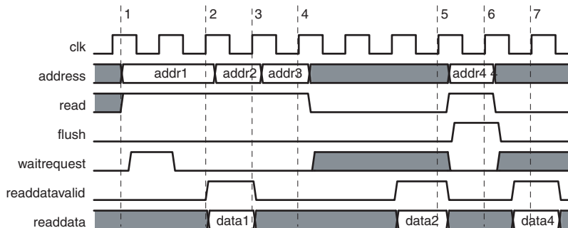
Figure 3.11. Master Pipelined Read Transfer
