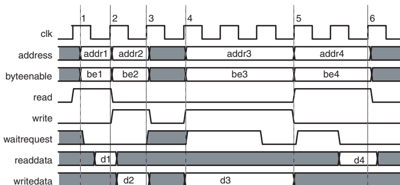
Figure 3.10. Fundamental Master Read and Write Transfers
