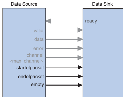
Figure 6.9. Avalon-ST Packet Interface Signals
