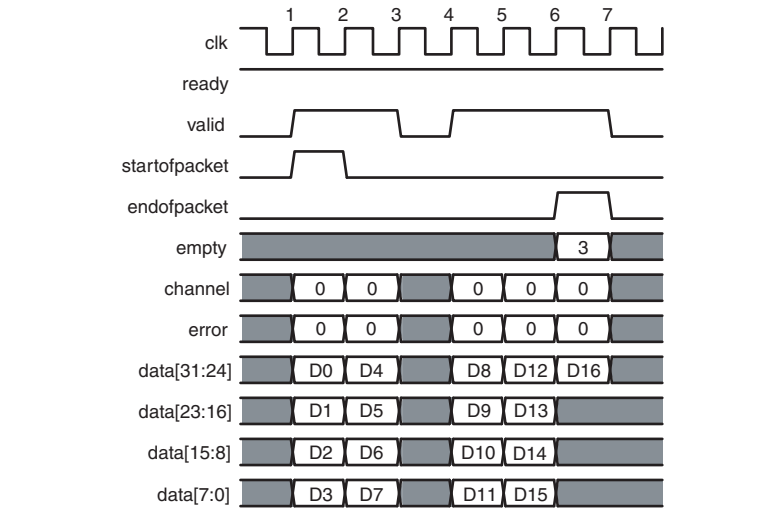
Figure 6.10. Packet Transfer
