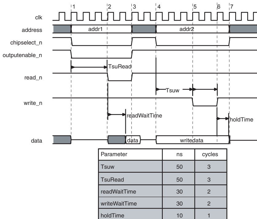
Figure 5.4. Tristate Slave Read and Write Transfers with Setup Time and Wait-States
