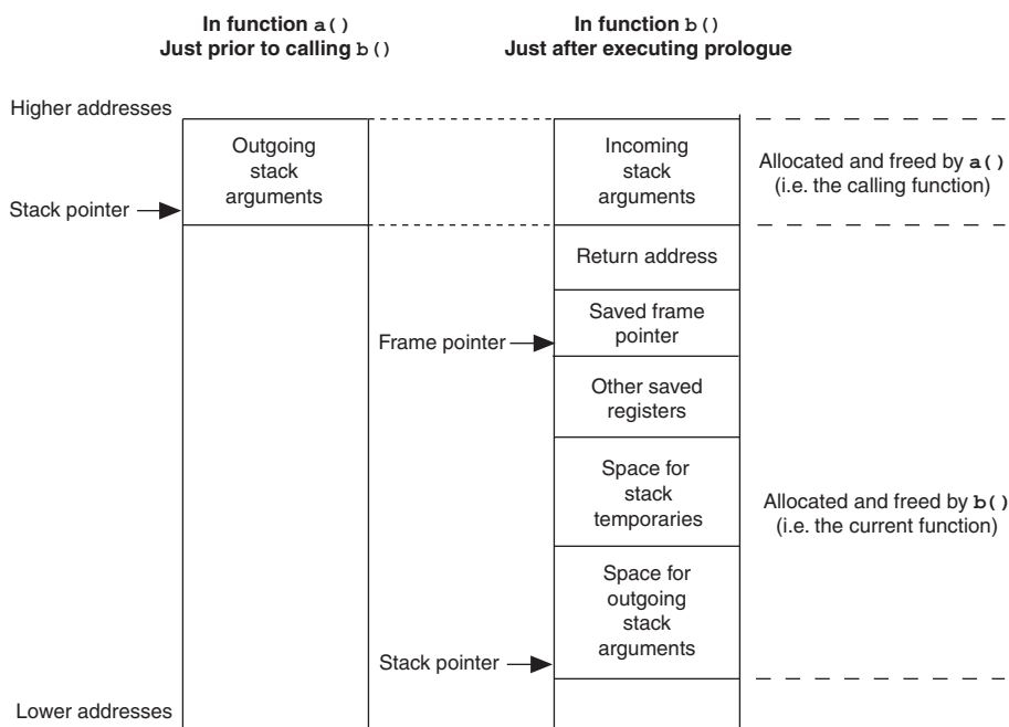
Figure 7-1. Stack Pointer, Frame Pointer and the Current Frame
