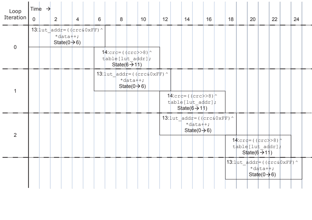
Figure 4–6. CRC Critical Path Scheduling by Assignment
