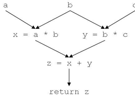
Figure 3–12. Dependency Graph
