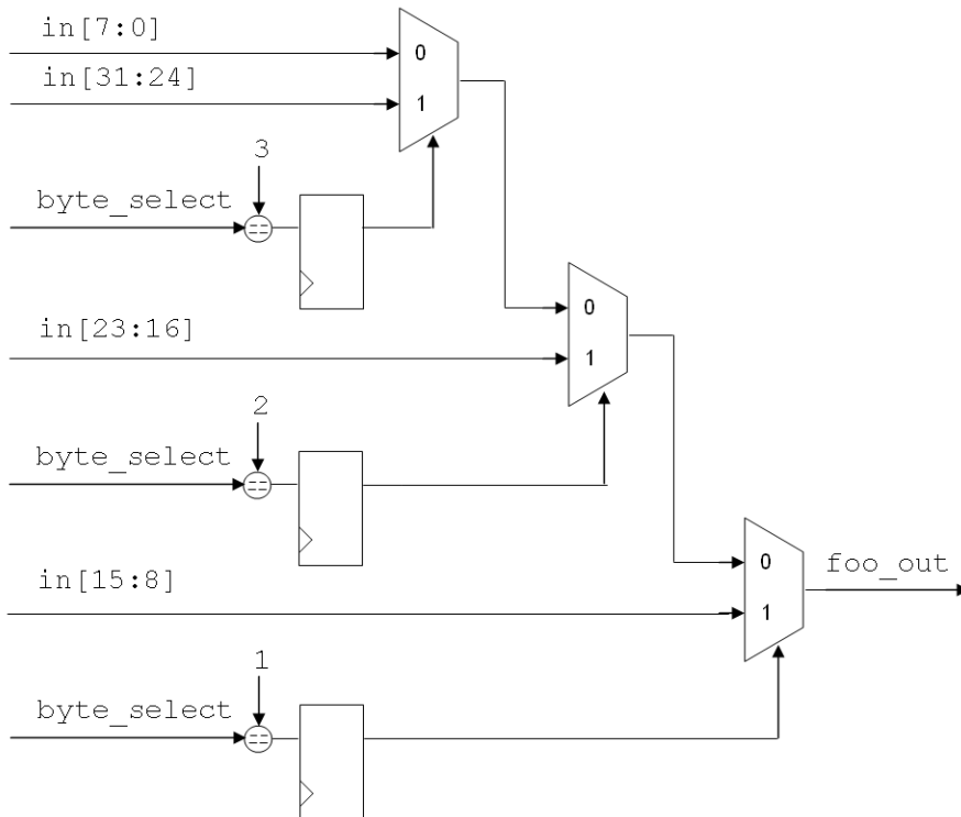
Figure 3–7. switch Logic
