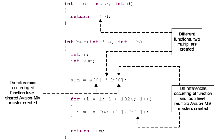
Figure 3–26. Shared And Independent Resources
