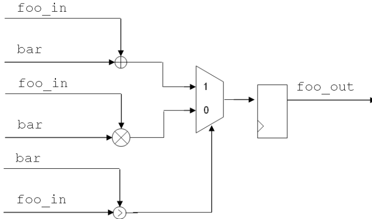
Figure 3–6. if-else Logic
