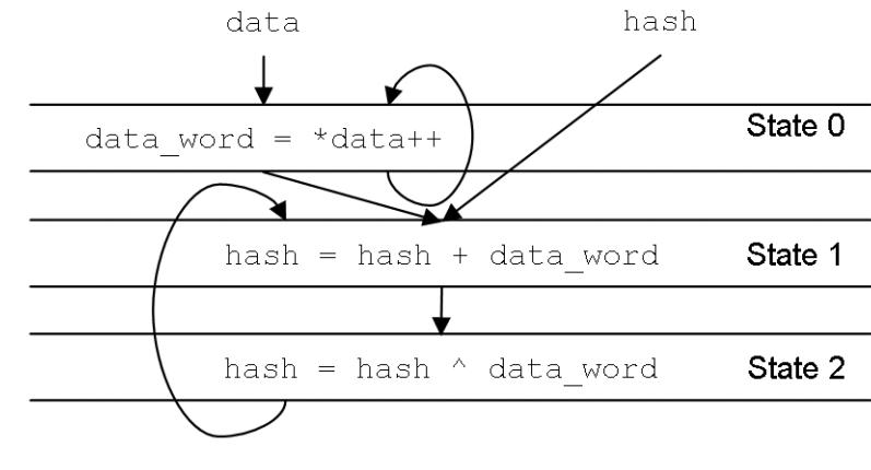
Figure 3–22. Loop-Carried Dependency
