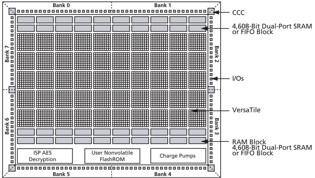
Figure 1 • Device Architecture Overview
