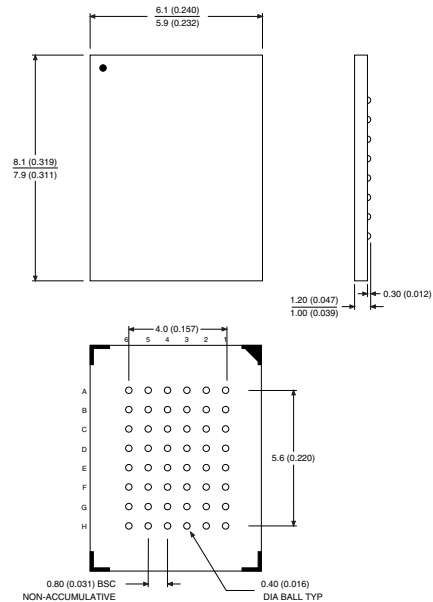
48C5 , 48-ball, Plastic Chip-size Ball Grid Array Package (CBGA) Dimensions in Millimeters and (Inches)*
