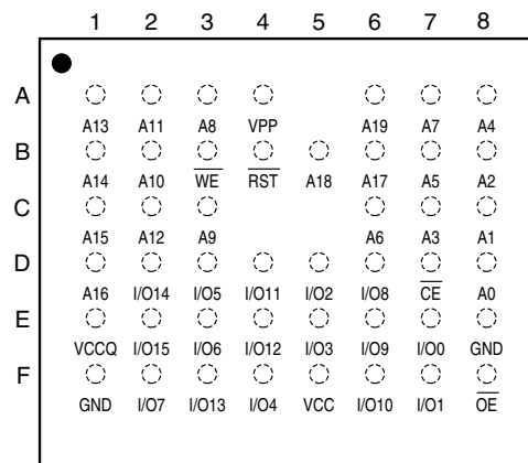
CBGA Top View (Ball Down)
