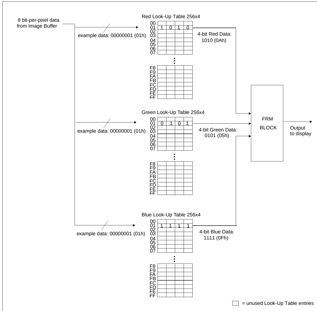
Figure 12-4: 8 Bit-Per-Pixel Color Mode Data Output Path
