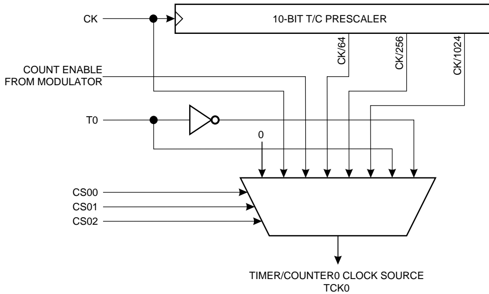
Figure 20. Timer/Counter0 Prescaler
