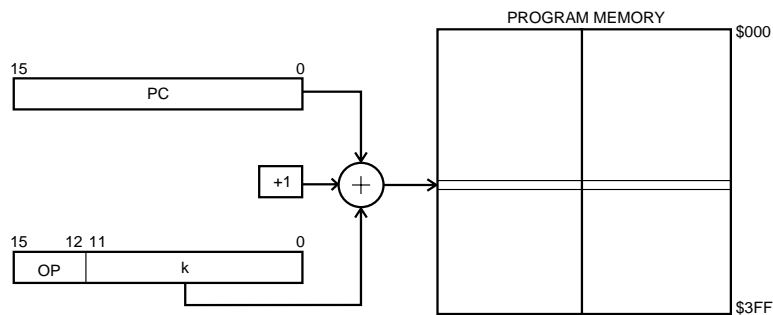
Figure 11. Relative Program Memory Addressing
