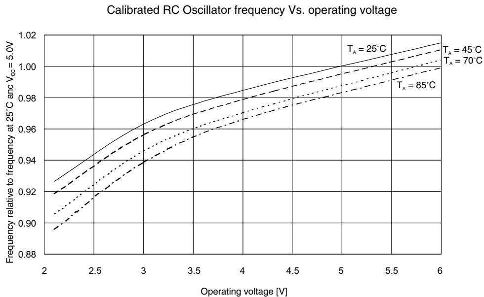
Figure 36. Calibrated Internal RC Oscillator Frequency vs. V_{CC}
