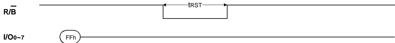
Figure 11. RESET Operation
