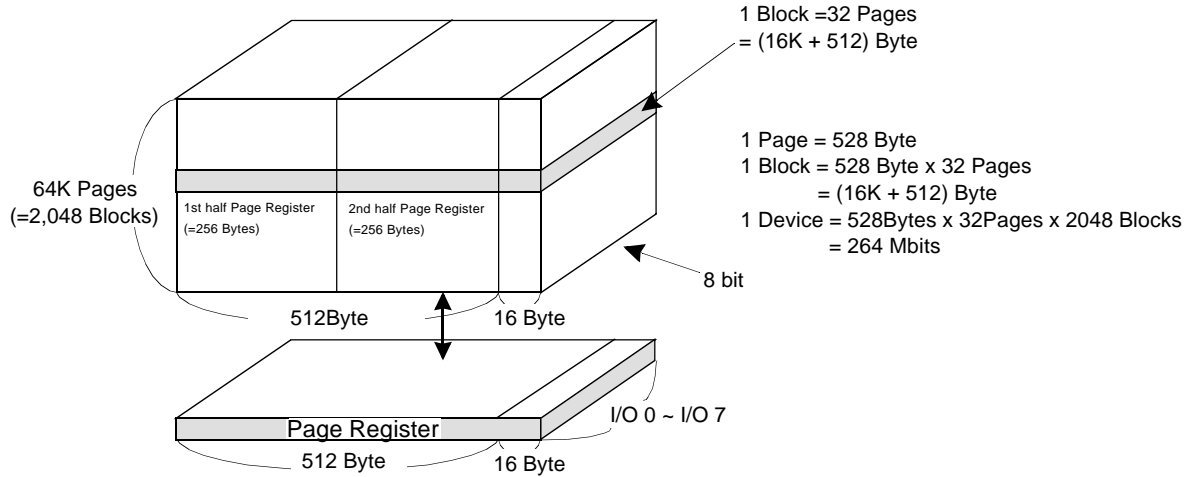
Figure 2. ARRAY ORGANIZATION
