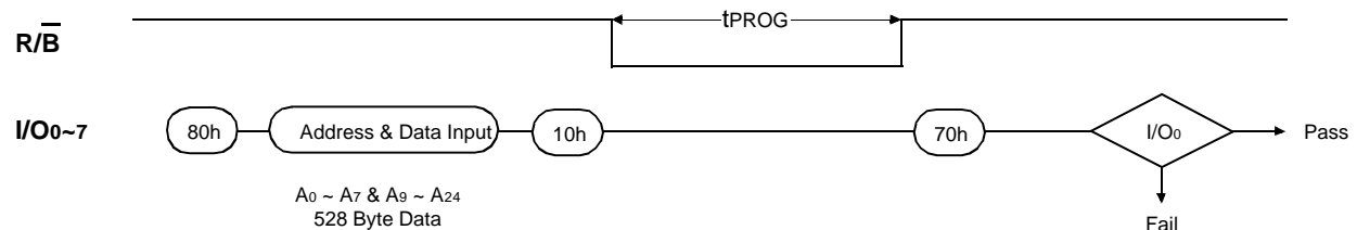
Figure 7. Program Operation
