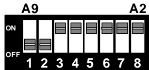
Figure 2 - DIP-Switch Illustration
