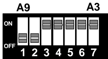
Figure 2 - DIP-switch Illustration
