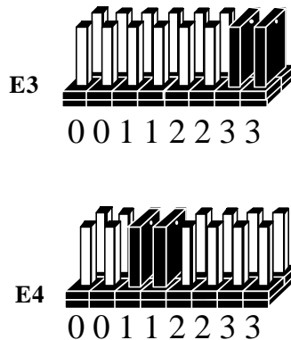
Figure 4 - DMA Selection Headers E3 & E4
