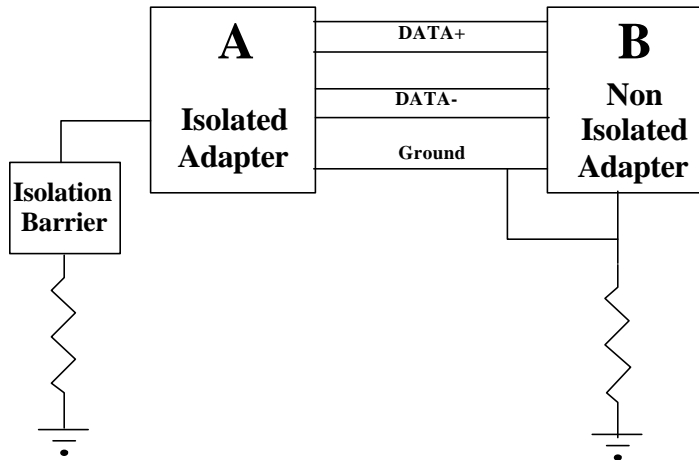
Figure 8 – ULTRA COMM+LPCI cabling example
