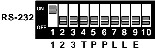
Figure 1 - RS-232
