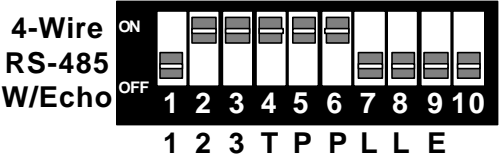
Figure 3 - RS-485, 4-Wire with Echo
