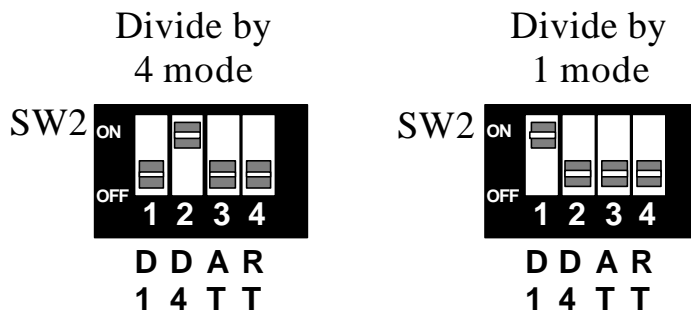
Figure 7 - Clocking Modes
